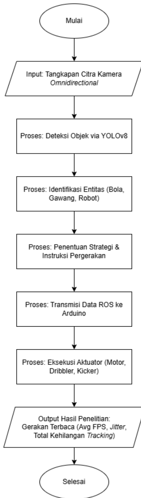
Gambar 3.3 Flowchart Kerja Sistem Baseline
